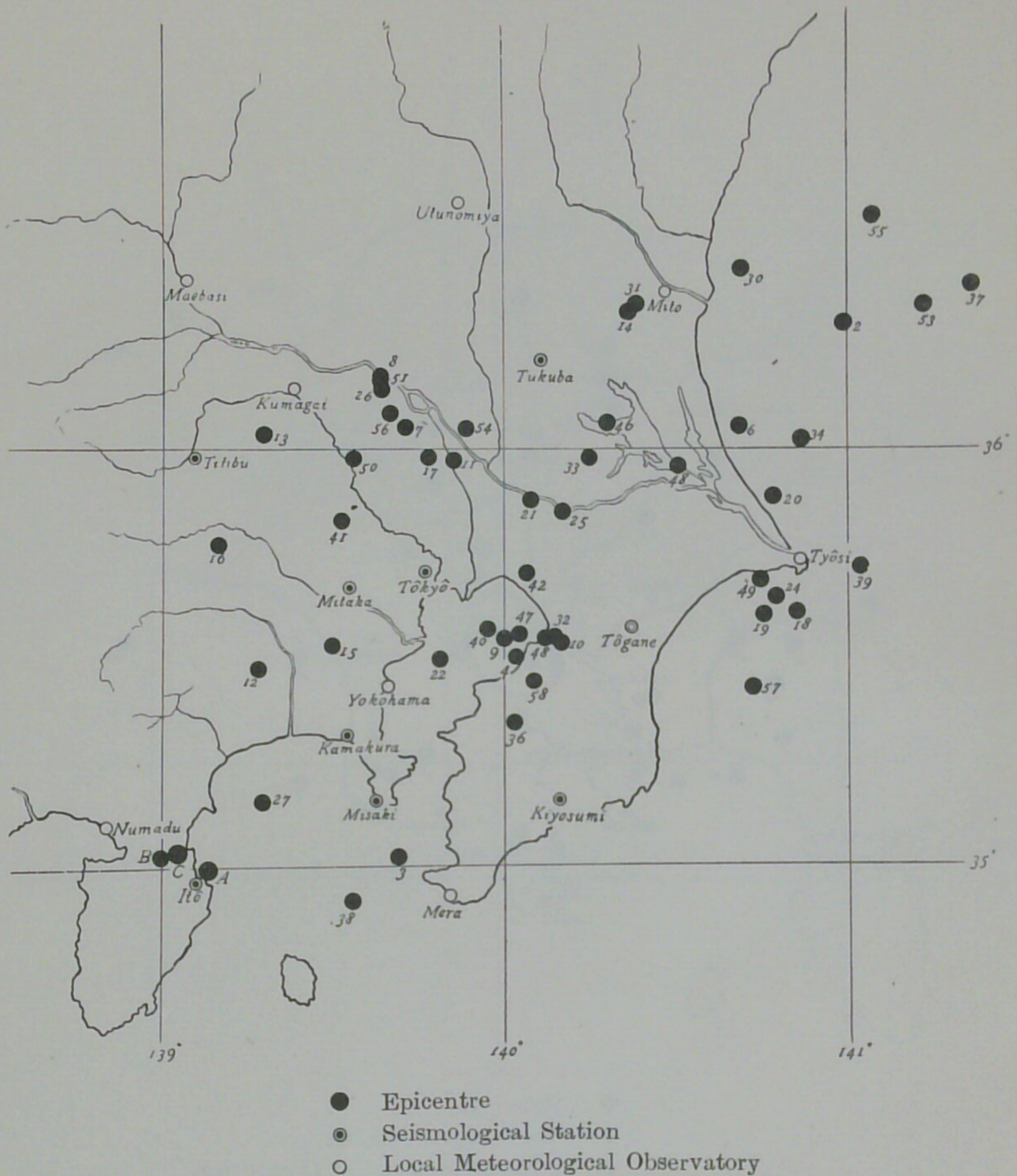
Fig. 7. Distribution of the earthquakes that originated within a distance of 160 kms. from Tōkyō and felt there in 1930. (Figures attached to each epicentre indicate the earthquake number in List VII. A, B, C indicate positions of the Itō swarm earthquakes, the destructive Idu earthquake and the Aziro swarm earthquakes respectively.)
