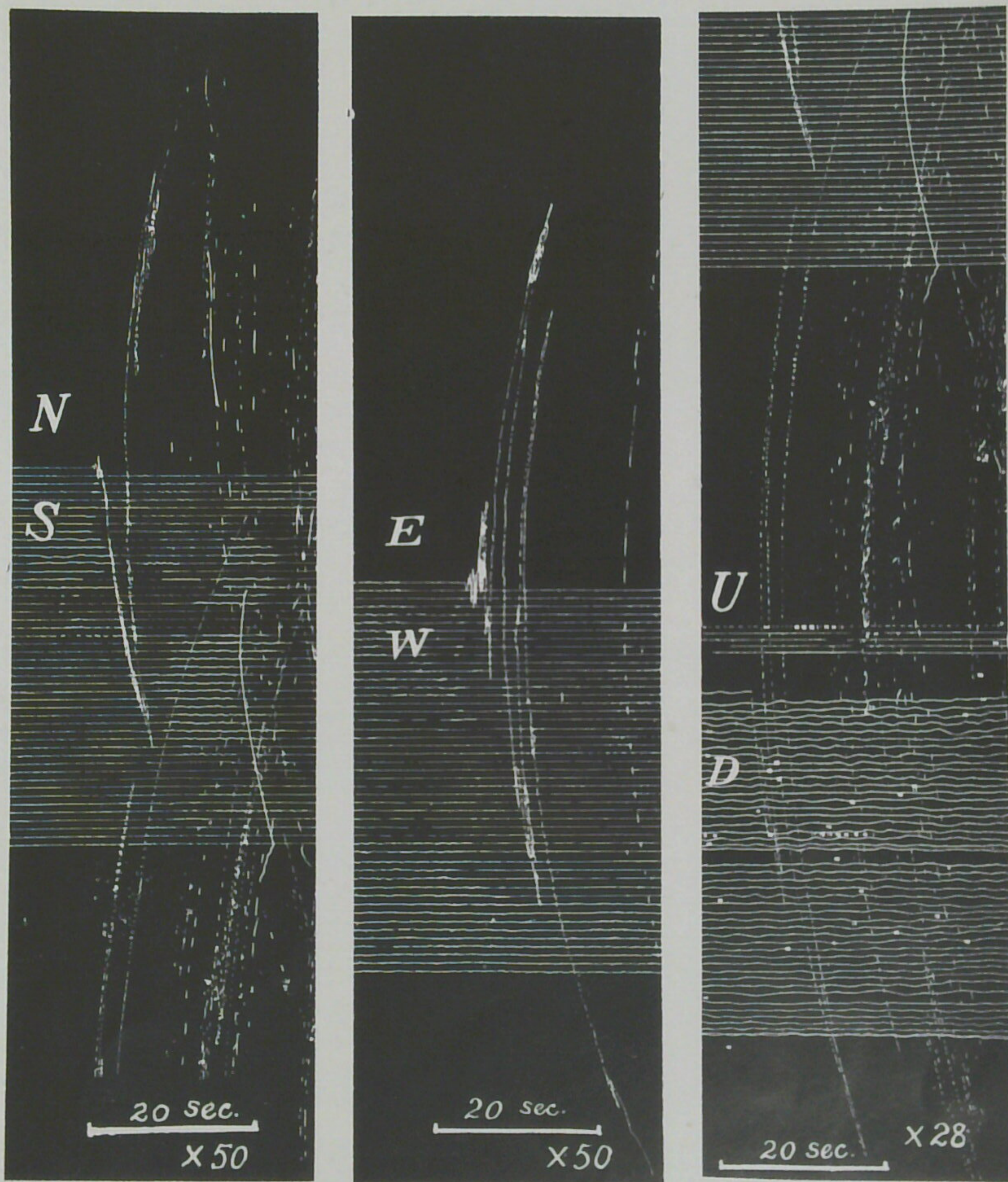
Fig. 7. Tôkyô Observation of the Strong Earthquake of June 17, 1931. Three Component Motions Seismograph Diagram.
