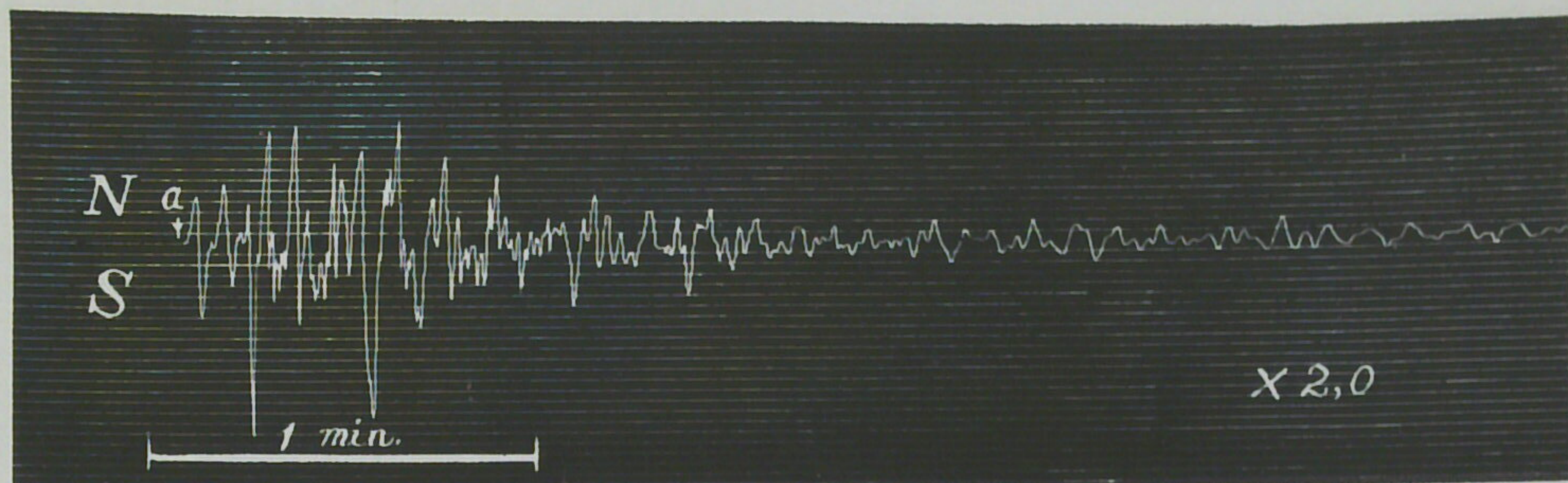
Fig. 8. Kamakura Observation of the Strong Earthquake of June 17, 1931. Strong Motion Seismograph Diagram.
