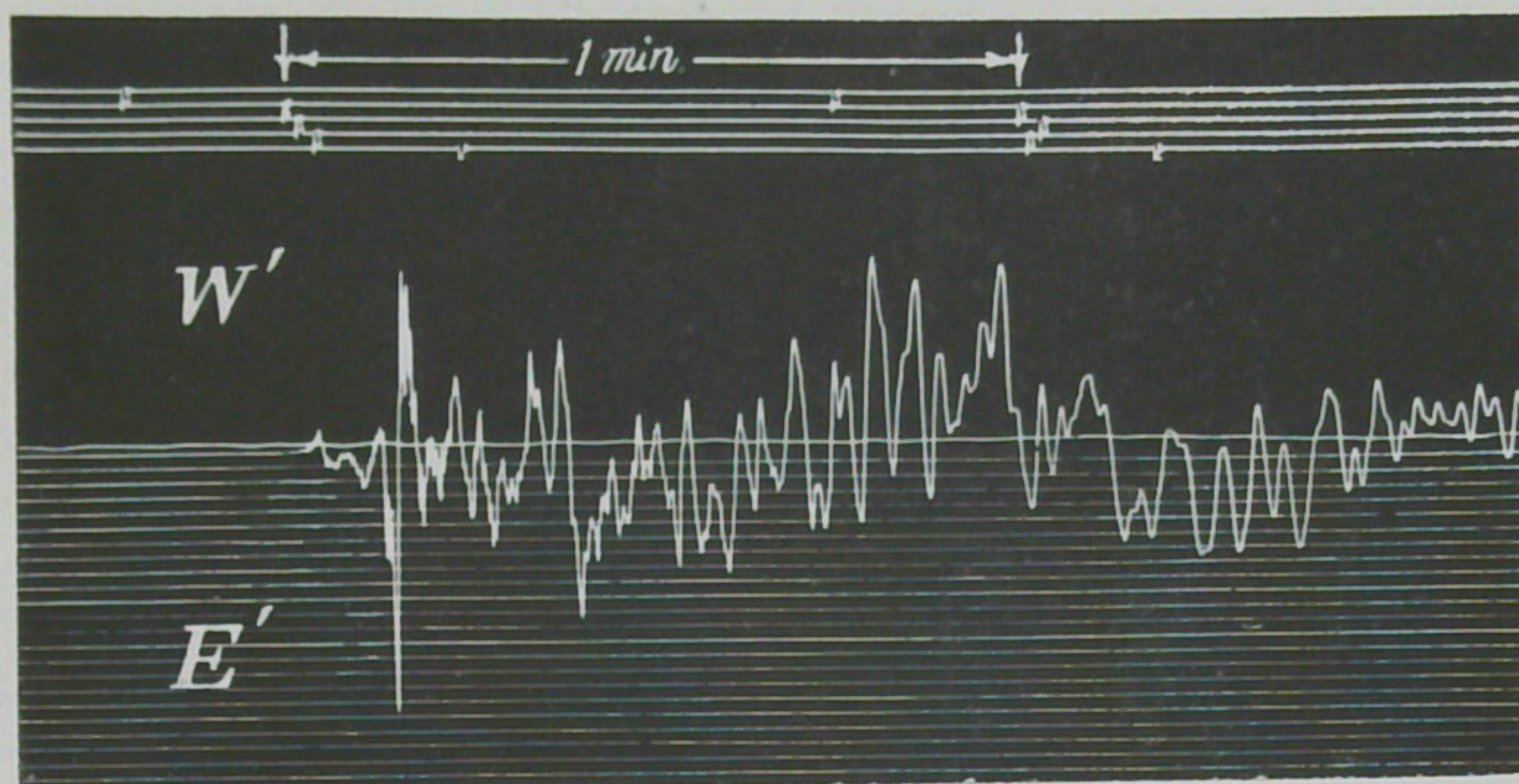
Fig. 5. Tôkyô (Hongô) Observation of the Strong Earthquake of June 17, 1931. Horizontal Pendulum Strong Motion Seismograph Diagrams.
