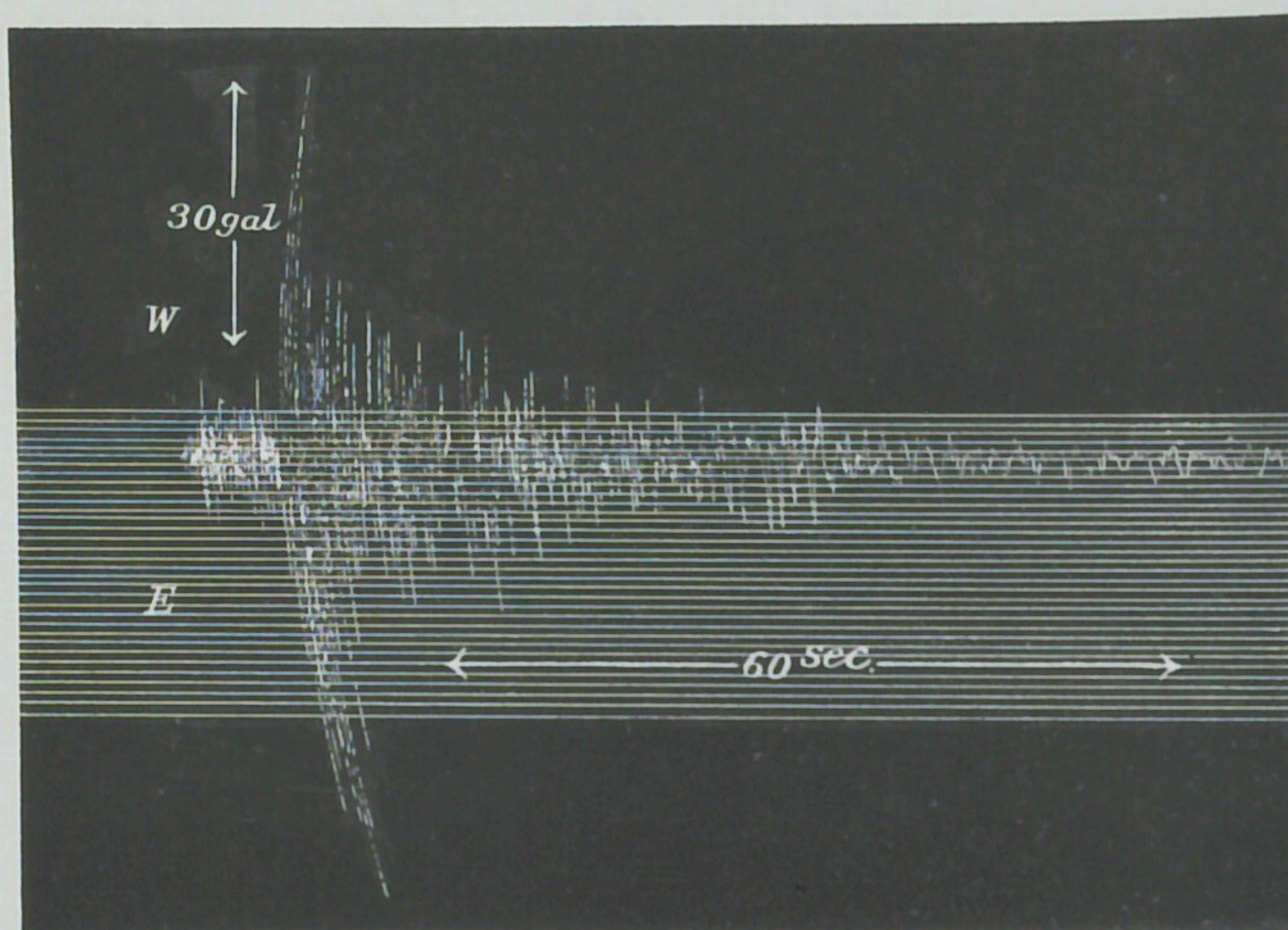
Fig. 11. Tôkyô (Hongô) Observation of the Strong Earthquake of June 17, 1931. Ishimoto Acceleration Seismograph Diagram.
